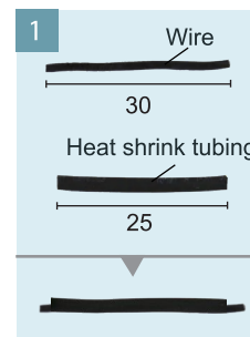
Insert wire into heat shrink tubing and heat the tubing to shrink.
