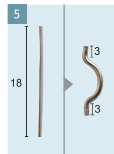
Cut and bend as shown.
